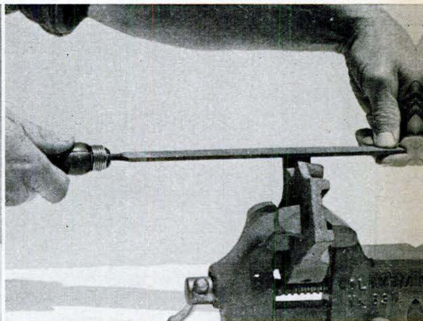
LIGHT FILING and finishing is done with a sensitive, two-finger grip on the end of the file. Lift file on return stroke.
